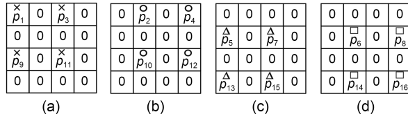
Fig. 7 Sample set graph obtained from preprocessing: (a) cross set C_1 ; (b) circle set C_2 ; (c) triangle set C_3 ; (d) square set C_4
