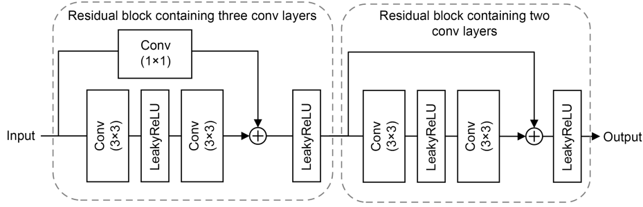
Fig. 3 Architecture of the residual group blocks
