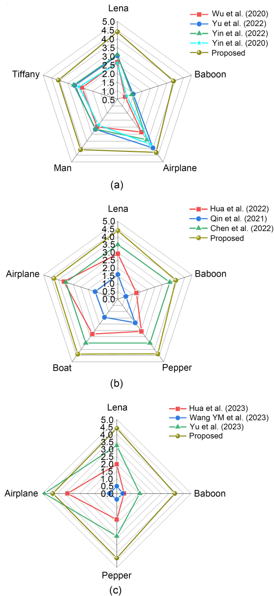
Fig. 14 Comparison of capacity with similar schemes: (a) comparison with methods (Wu et al., 2020; Yin et al., 2022; Yu et al., 2022) on Lena, Baboon, Airplane, Man, and Tiffany; (b) comparison with methods (Qin et al., 2021; Chen et al., 2022; Hua et al., 2022) on Lena, Baboon, Pepper, Boat, and Airplane; (c) comparison with methods (Hua et al., 2023; Wang YM et al., 2023; Yu et al., 2023) on Lena, Baboon, Pepper, and Airplane
