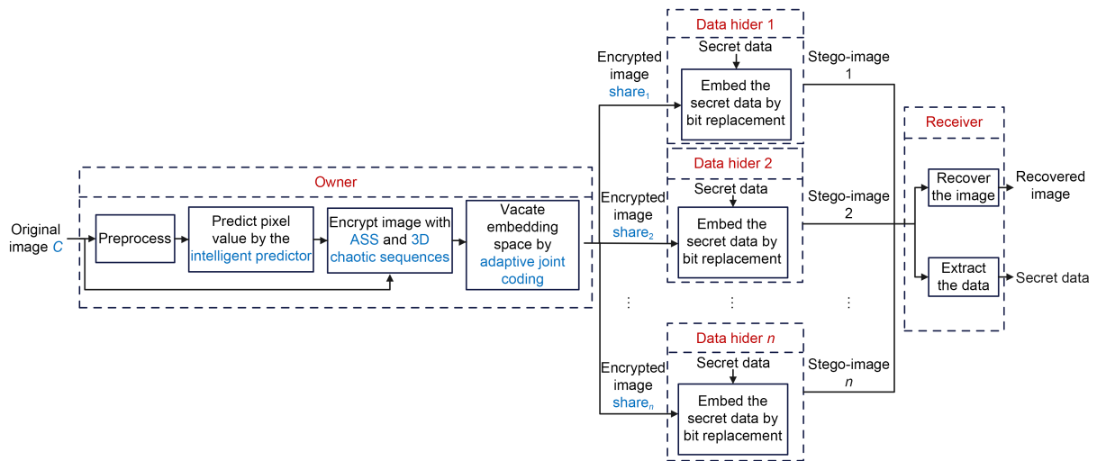
Fig. 6 An overview of the proposed reversible data hiding in encrypted images (ASS: additive secret sharing)
