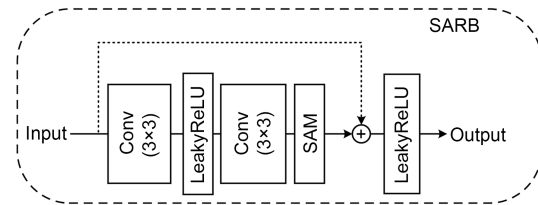
Fig. 2 Architecture of SARB (SARB: spatial attention residual block; SAM: spatial attention module)
