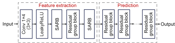
Fig. 1 Architecture of the proposed predictor (SARB: spatial attention residual block)
